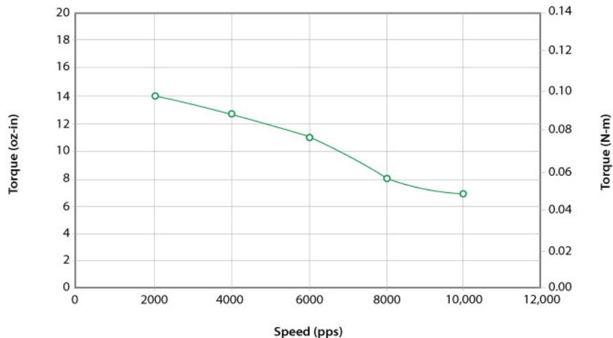
3709V-18 24VDC, 0.6 Amps/Phase, Bipolar, 1/2 Stepping
