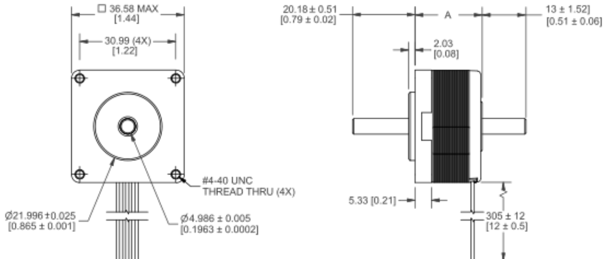
3709V-18 24VDC, 0.6 Amps/Phase, Bipolar, 1/2 Stepping
